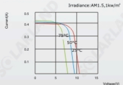
SLP003-06 I-V Curves
