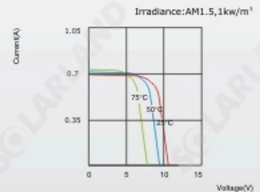
SLP005-06 I-V Curves
