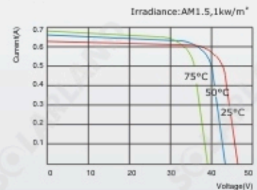
SLP020-24 I-V Curves
