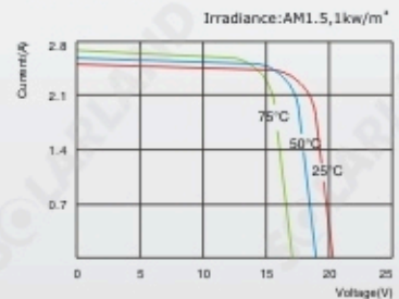
SLP040-12 I-V Curves
