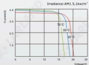
SLP060-12 I-V Curves
