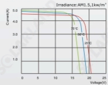
SLP075-12 I-V Curves
