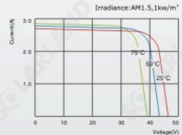
SLP085-24 I-V Curves
